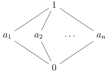
Figure 2.1: M_n
