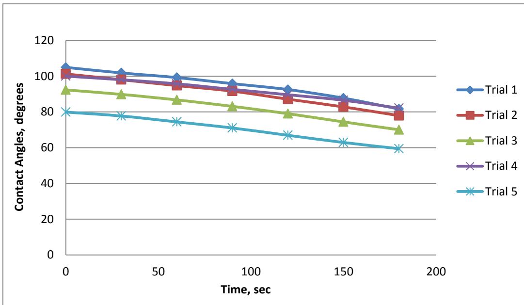
FIGURE 62- PP Soaked in EcoSurf for 20 Min
