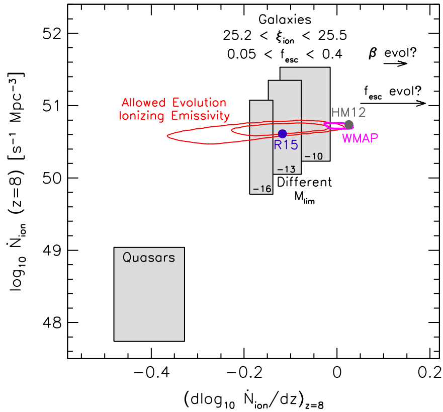
Figure 7. 68% and 95% confidence intervals on parameters describing the cosmic ionizing emissivity (assuming C_{\text{H II}} = 3 : red contours) and a comparison to the emissivity expected (gray boxes in the upper middle) for galaxies to three different faint-end cut-offs to the LF ( -10 , -13 , and -16 mag) where the Lyman-continuum photon production efficiency \xi_{\text{ion}} and f_{\text{esc}} plausibly have values over the wide range: 10^{25.2}-10^{25.5} \text{ s}^{-1}/(\text{erg s}^{-1} \text{ Hz}^{-1}) and 0.05-0.40 based on the observations (e.g., Siana et al. 2010, 2015; Vanzella et al. 2012; Mostardi et al. 2013; Bouwens et al. 2014; Cooke et al. 2014). The arrows indicate how potential evolution in the UV-continuum slopes \beta 's or f_{\text{esc}} of galaxies (as d\beta/dz \sim -0.04 [predicted by Wilkins et al. 2013 and consistent with the evolution observed by Bouwens et al. 2014] or f_{\text{esc}} \propto (1+z)^{3.4} : required by HM12 to match the WMAP \tau measurements) would affect the evolution of \dot{N}_{\text{ion}} . The gray box to the lower left shows the expectations for quasars using the Willott et al. (2010) results to set the normalization of the ionizing emissivity \dot{N}_{\text{ion}}(z) (after correcting their results upwards by 0.2 dex to account for a possibly steeper faint-end slope \alpha \sim -2 vs. the \alpha = -1.5 Willott et al. 2010 adopt) and the redshift dependence of the emissivity from the McGreer et al. (2013) LEDE and modified LEDE models. The 68% likelihood contours preferred based on the WMAP optice depths and assuming reionization finishes at z = 5.9-6.5 are shown in magenta. The small size of the WMAP contours is an artifact of the sensitivity of the computed optical depths \tau to small changes in (d \log_{10} \dot{N}_{\text{ion}}/dz)_{z=8} when (d \log_{10} \dot{N}_{\text{ion}}/dz)_{z=8} approaches 0 (since such implies a constant \rho_{\text{UV}} to arbitrarily high redshift). The gray and blue circles give the equivalent parameters from the HM12 and R15 models, respectively. It is clear that galaxies should be successful at producing the inferred ionizing emissivity for a variety of plausible values for f_{\text{esc}} , \xi_{\text{ion}} , and M_{\text{lim}} . It is also clear from this figure that quasars/AGN seem quite unlikely to be the source of this emissivity (see also HM12).
