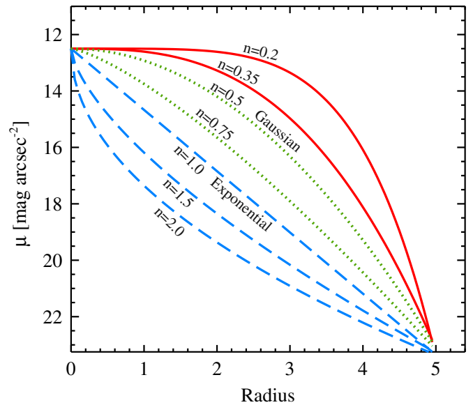
Figure 1. Schematic plot of Sérsic profiles that describe various radial surface brightness profiles of bars. Radial profiles of n = 0.2 – 2.0 are presented. Gaussian ( n = 0.5 ) and exponential ( n = 1.0 ) profiles are also shown. Flat profiles are in red, intermediate profiles are in green, and exponential steep profiles are in blue. Radius is in an arbitrary unit.
