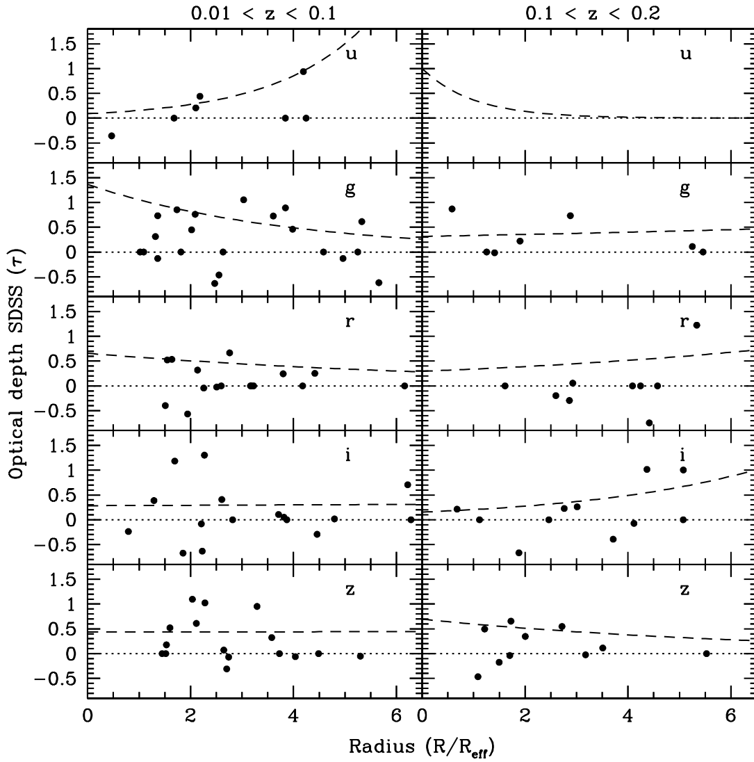
FIG. 7.— Radial opacity plot in all five SDSS filters ( u' , g' , r' , i' , and z' ) for the redshift ranges z = 0.01\text{--}0.1 and 0.1\text{--}0.2 for the foreground spiral disks. Radii are scaled by the half-light radius ( R_{\text{eff}} ). The opacity measurements are done in the visually determined aperture. Dashed lines are the exponential fits to the opacity measurements.
