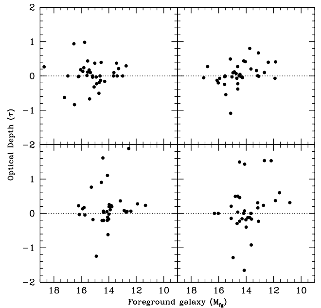
FIG. 8.—Plot of disk optical depth and foreground galaxy magnitude, measured by the Source Extractor run part of the fit. There appears to be little relation between optical depth and disk brightness, probably because other effects—radial distance, arm presence, and Hubble type—dominate the optical depth value. Negative optical depth values occur when there is significant asymmetry in either or both of the members of the occulting pair.
