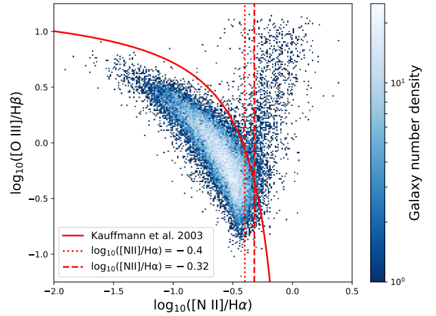
Figure 3. A BPT diagram of the emission line galaxies in GAMA. The Kauffmann et al. (2003) line is plotted as the solid red curve. The red dotted line shows \log_{10}([\text{N II}]\lambda 6583/\text{H}\alpha) = -0.4 , often used to select AGN in WHAN diagnostic criteria. The red dashed line shows \log_{10}([\text{N II}]\lambda 6583/\text{H}\alpha) = -0.32 used to select AGN in this work. The large fraction of star forming galaxies located between the two vertical lines is readily apparent.
